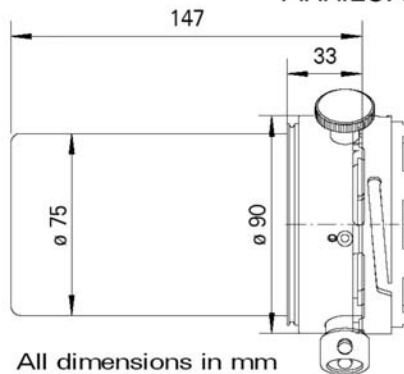
ARRILUX 400 Lighthouse
